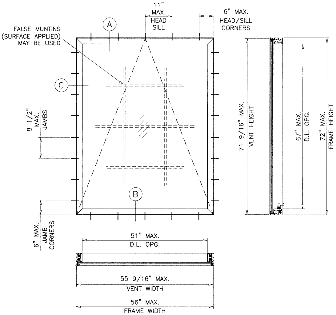
TYPICAL ELEVATION
